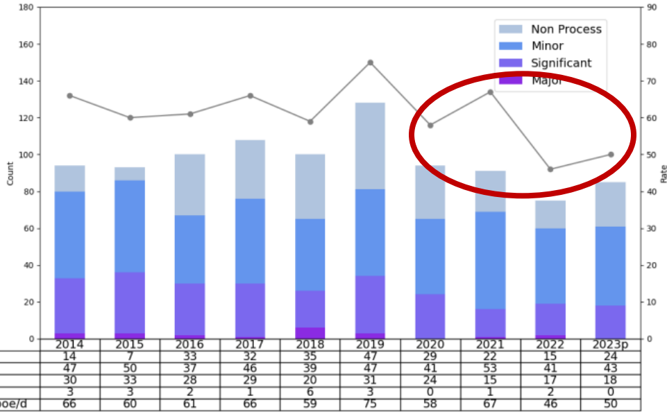
Figure 9. Hydrocarbon Releases (offshore) 2014-2023p
